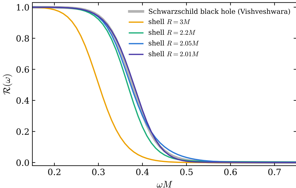
Odd parity, \ell = 2 : shell \rightarrow black hole as R \rightarrow 2M
